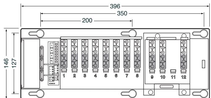
Fixing points M6 (1/4")
